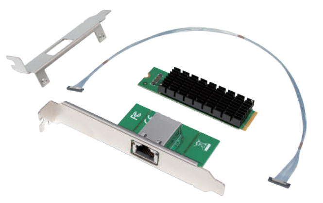
RJ45 Board: 38 x 60 mm
