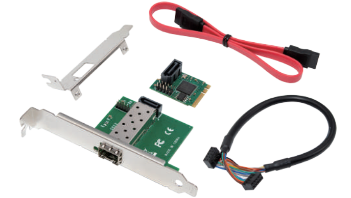
SFP Board: 52 x 63 mm
