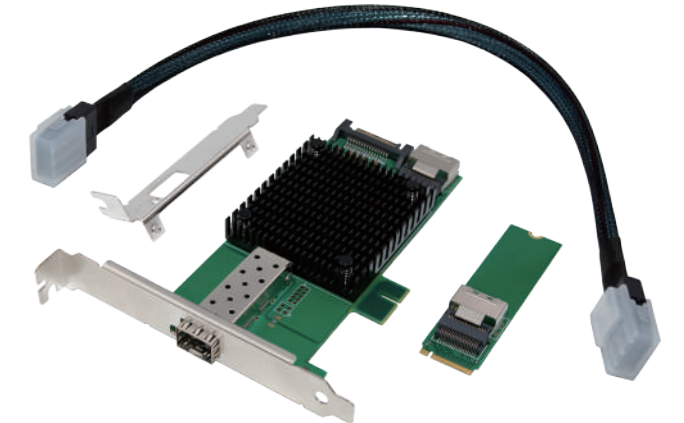
SFP+ Board: 130 x 68 mm
