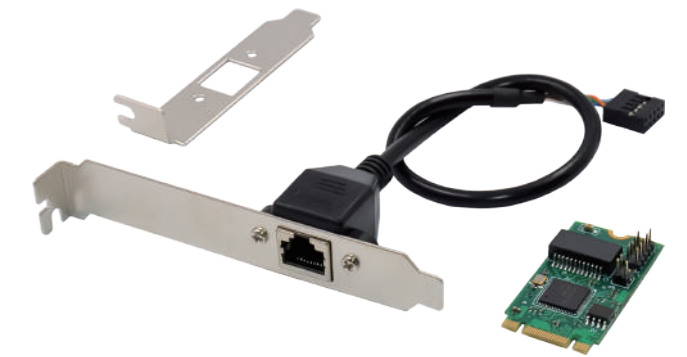
RJ45 Port: L35 x W21 x H22 mm
