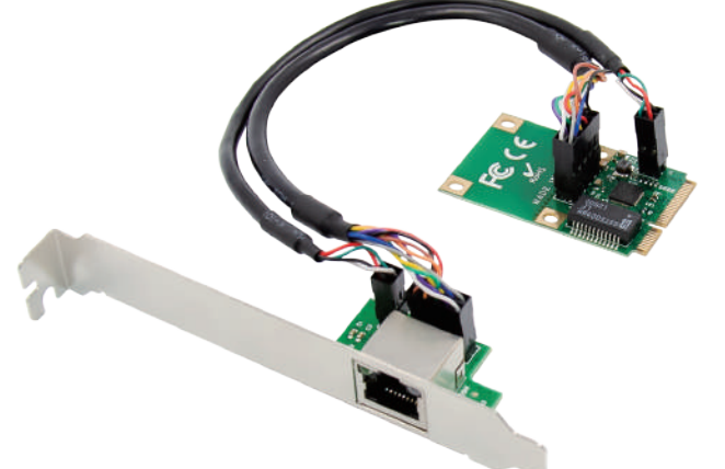
RJ45 Board: L25 x W38 x H15 mm
