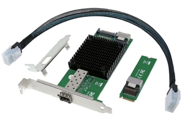
SFP+ Board: 130 x 55 mm
