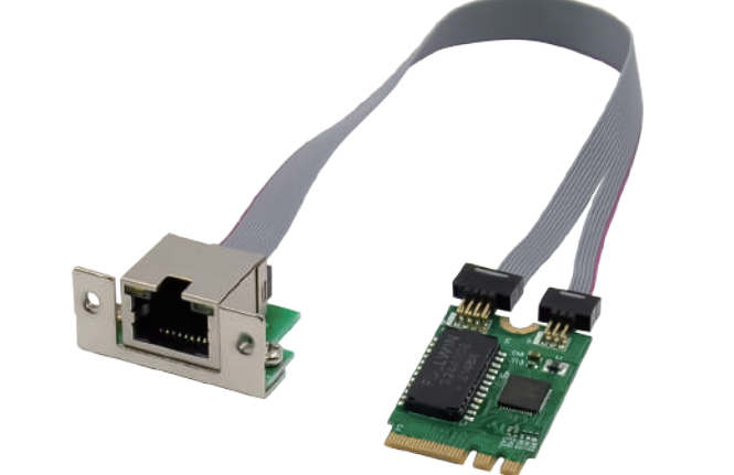
RJ45 Board: L30 x W20 x H15 mm
