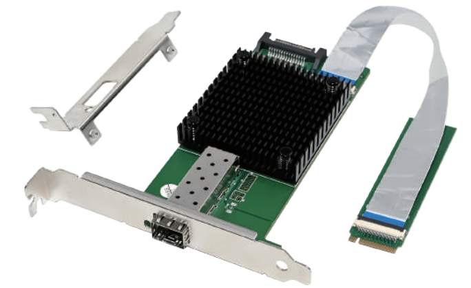
SFP+ Board: 130 x 55 mm
