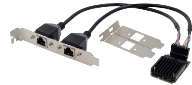
RJ45 Port: L35 x W21 x H22 mm
