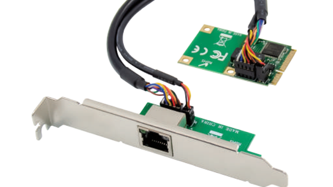
RJ45 Board: 25 x 63 mm
