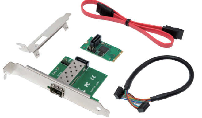
SFP Board: 52 x 63 mm
