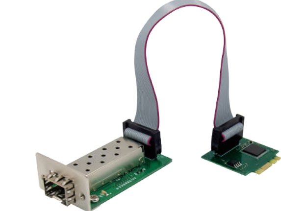
SFP Board: 52 x 63 mm
