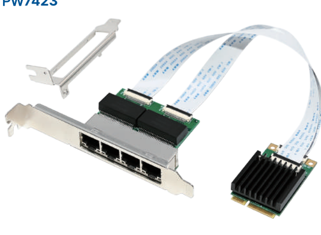
RJ45 Board: 52 x 63 mm
