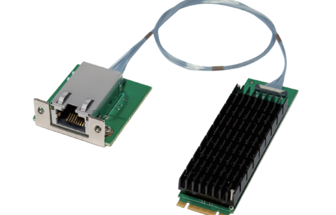
RJ45 Board: 38 x 35 mm
