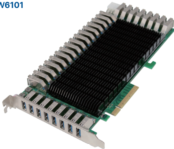
PCIe x8 NEC720201 32 * USB3.0 Camera Capture Card
